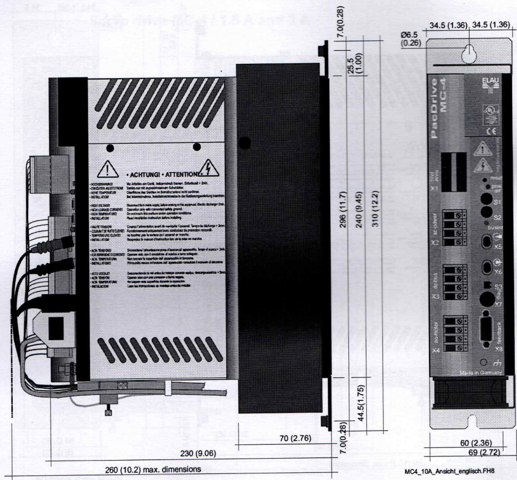
Fig. 4-3: Dimensions of the MC-4 / 10 A
