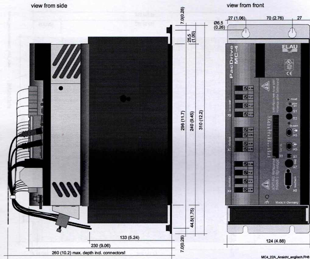
Fig. 4-4: Dimensions of the MC-4 / 22 A
