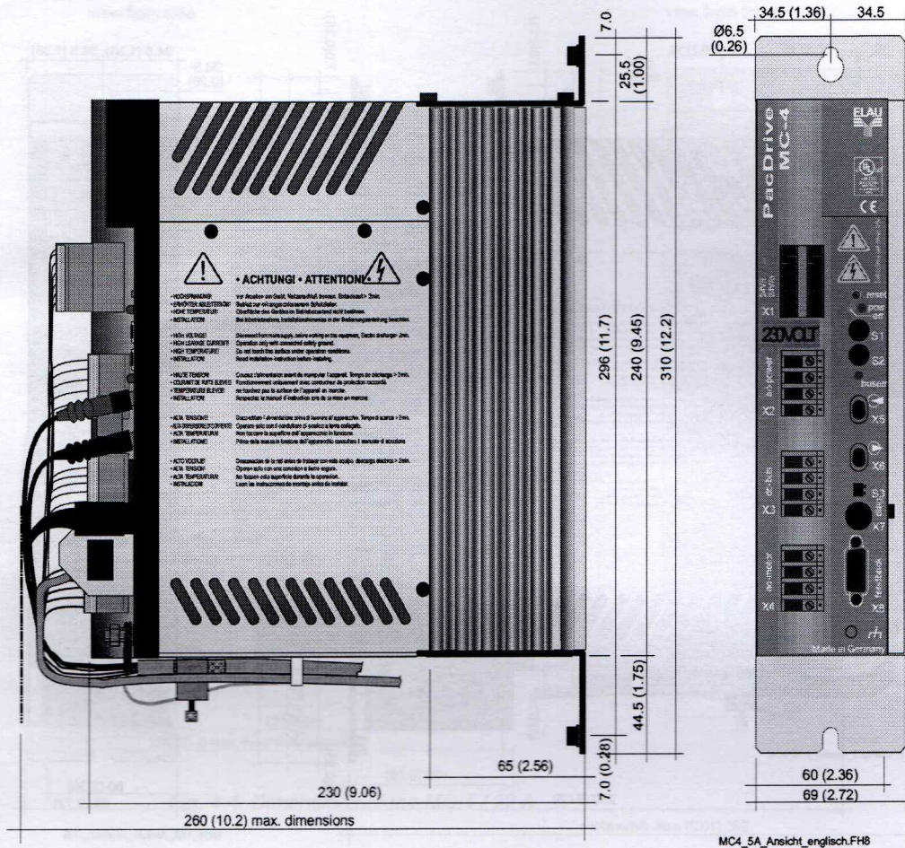
Fig. 4-2: Dimensions of the MC-4 / 5 A
