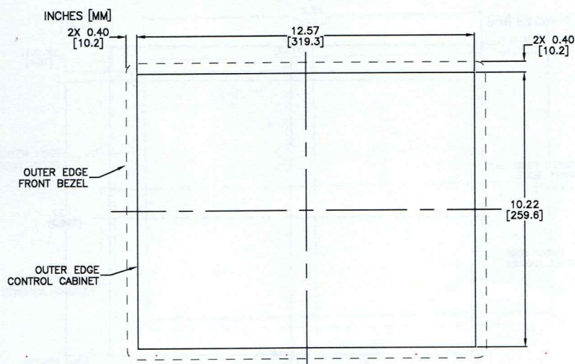
PANEL CUTOUT
