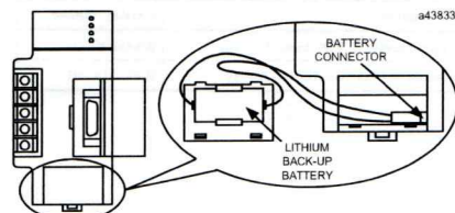
Figure 5. Location of PLC RAM Memory Backup Battery
