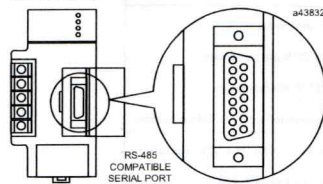
Figure 4. Serial Port Connector
