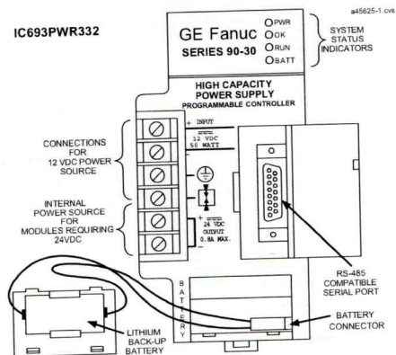
Figure 1. Series 90-30, 12 VDC Input, High Capacity Power Supply - IC693PWR332
