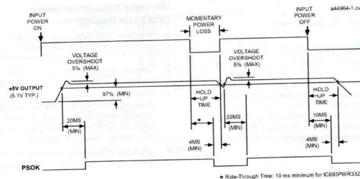
Figure 3. DC Power Supply Timing Diagram
